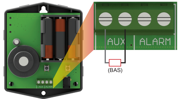
(Fig. 7; auxiliary contacts)
