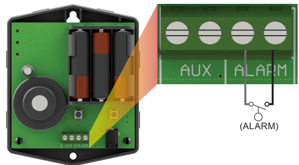
(Fig. 8; sensor/signaling device)
